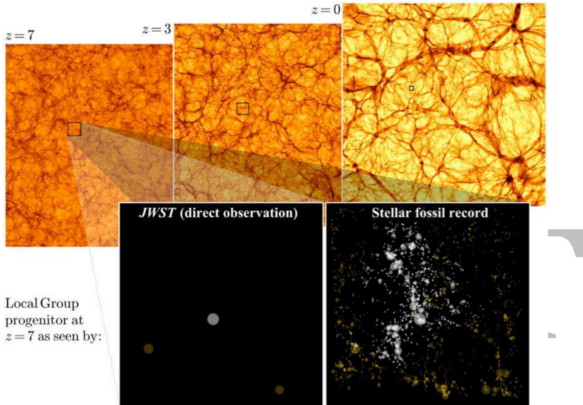
Figure 33: Density slices of the Illustris simulation at different redshifts, each with a side length of 106.5 co-moving Mpc. The square in each panel indicates the co-moving size of a Local Group-type structure at each redshift. These are comparable in size to the HST Ultra-Deep Field. The zoom-in panels show an expected image of the galaxies visible at z = 7 \pm 0.02 using JWST (left panel), and through the stellar fossil record in the Local Group (right panel; white symbols indicate structures still present in the Local Group at z = 0 , whereas gold symbols represent objects that are no longer present in the Local Group at z=0 ). (Figure from Boylan-Kolchin et al. 2015 ).
