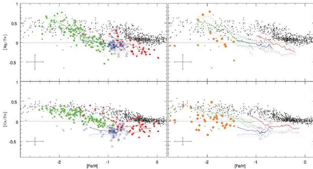
Figure 27: Alpha elements as a function of [\text{Fe}/\text{H}] in a variety of nearby dwarf galaxies. Left panel: Sagittarius (red/gray filled squares: Sbordone et al. 2007; McWilliam & Smecker-Hane 2005), Fornax (blue/dark-gray open triangles: Letarte et al. 2010) and Sculptor (green/light-gray filled circles: Hill et al. 2012). Right panel: Sextans (orange/light-gray filled circles: Kirby et al. 2010; Aoki et al. 2009; Shetrone et al. 2003). In all panels, solid lines show the average trend and dotted lines show the 1\text{-}\sigma dispersion for each dwarf galaxy. The underlying points show stars in the Milky Way (Cayrel et al. 2004; Venn et al. 2004). (Figure from Hill et al. 2012).
