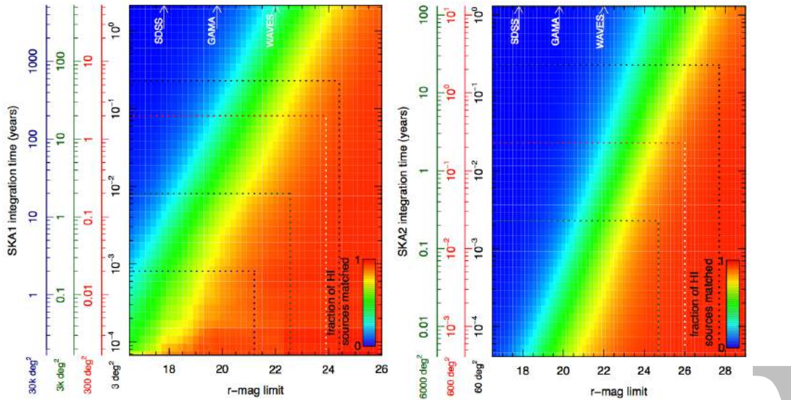
Figure 12: Fraction of HI SKA survey sources (left panel, SKA1; right panel, SKA2) that are detected in an r-band apparent magnitude-limited sample. For SKA1, four surveys are considered (including the now defunct SKA-SUR mode): 3 deg 2 using SKA1-MID (black), 300 deg 2 using SKA1-SUR (red), 3000 deg 2 using SKA1-SUR (green), and 30000 deg 2 using SKA1-SUR (blue). For SKA2, three surveys are considered: 60 deg 2 (black), 600 deg 2 (red), and 6000 deg 2 (green). Dotted lines indicate the r-magnitude limit needed to achieve matches for 90% of sources in each SKA survey area (given 2000 hrs of integration for SKA1-MID & SKA2 surveys, and 2 years of telescope time for SKA1-SUR surveys). Dashed lines indicate 90% completion thresholds. Figure from Meyer et al. (2015).
