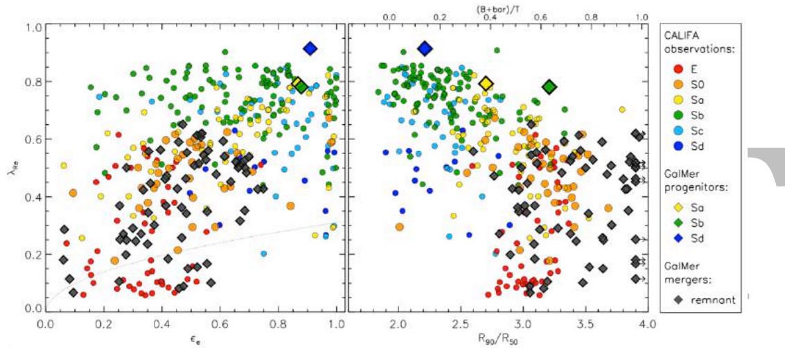
Figure 57: \lambda_R vs. ellipticity (left) and concentration ( C = R_{90}/R_{50} ) (right) for CALIFA galaxies, colour coded by morphology (circles). These are compared to remnant galaxies in merger simulations (diamonds). (Figure from Querejeta et al. 2015).
