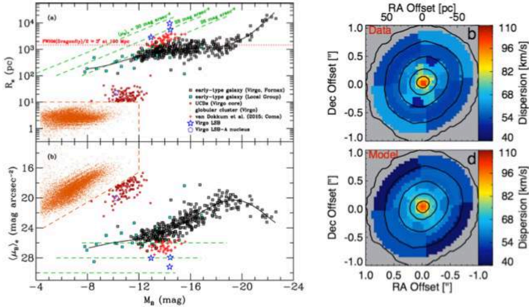
Figure 50: Left panel: Magnitude–size–surface brightness relations for a collection of dynamically hot stellar systems, mostly in the Virgo and Fornax clusters (Figure from Mihos et al. 2015). Right panel: Comparison of the observed and simulated two-dimensional velocity dispersion map for M60-UCD1, one of the most massive UCDs currently known. The central velocity dispersion “spike” is the signature of a 21 million solar mass black hole embedded in this low-mass ( 1.2 \times 10^8 M_\odot ) and compact ( R_e = 24 pc) stellar system (Figure from Seth et al. 2015).
