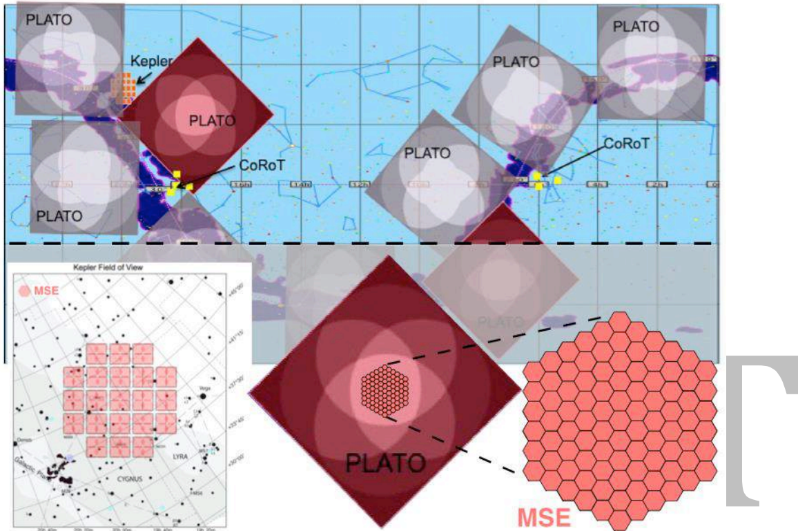
Figure 13: Top panel: schematic diagram showing the possible layout of the PLATO observing fields, relative to CoRoT and Kepler, in celestial coordinates, from Rauer et al. (2014). The PLATO field of view is 48.5 \times 48.5 square degrees, and it will observe roughly half the sky to m_V \sim 16 . The area above the dashed line is easily accessible to MSE (roughly \frac{1}{3} of the PLATO fields, or \sim 15000 square degrees). MSE can observe the faint end of the PLATO target distribution at high spectral resolution ( R \sim 40000 ) and very high SNR ( \sim 100 ) in short exposures ( < 300 s), with a velocity precision of order \sim 100 m/s. Possible observing strategies for MSE in the field of exoplanetary hosts include (a) covering all of the PLATO targets with single exposures; (b) targeting the Kepler survey fields, which will still have limited spectral coverage at the faint end in the 2020s. In the lower left panel, we show that the total \sim 115 square degree survey area can be covered, with high spatial completeness, in 84 MSE pointings; (c) a monitoring campaign of a subset of PLATO targets. In the lower right panels, we show a possible layout of 91 MSE fields covering the central 136 square degrees of the northern PLATO long duration field (that would take MSE about 8 hours to observe). (Figure adapted from Rauer et al. 2014).
