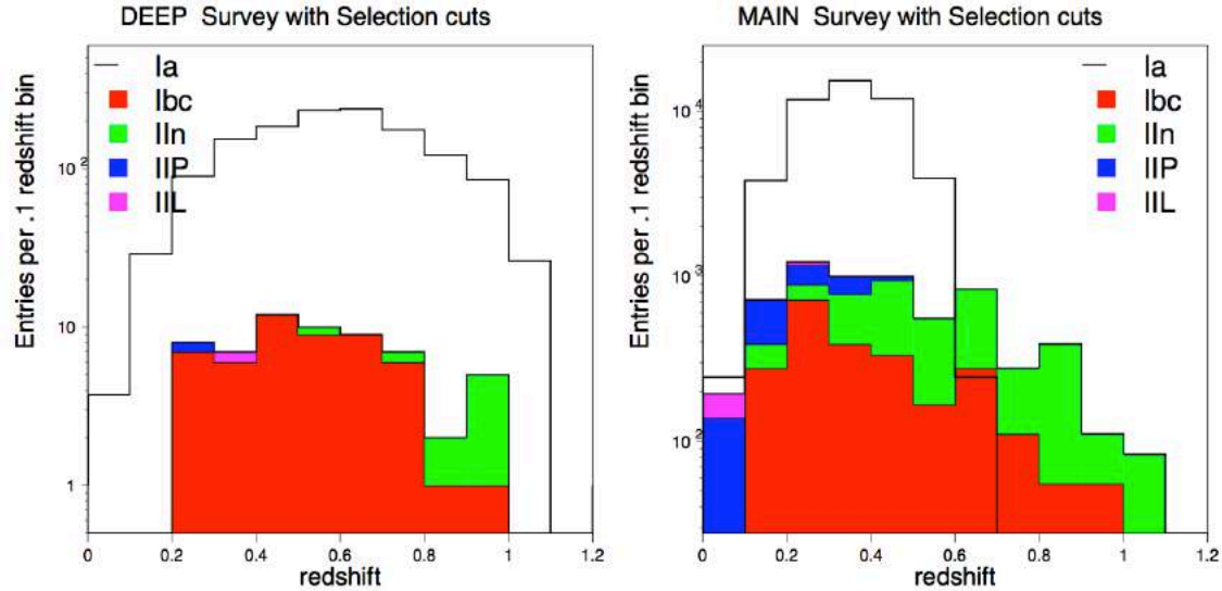
Figure 80: Predicted rates of Type Ia and non-Ia supernovae as a function of the redshift detected by LSST in the DEEP survey field (left panel) and the main survey (right panel). (Figure from The LSST Science Book v2 ).
