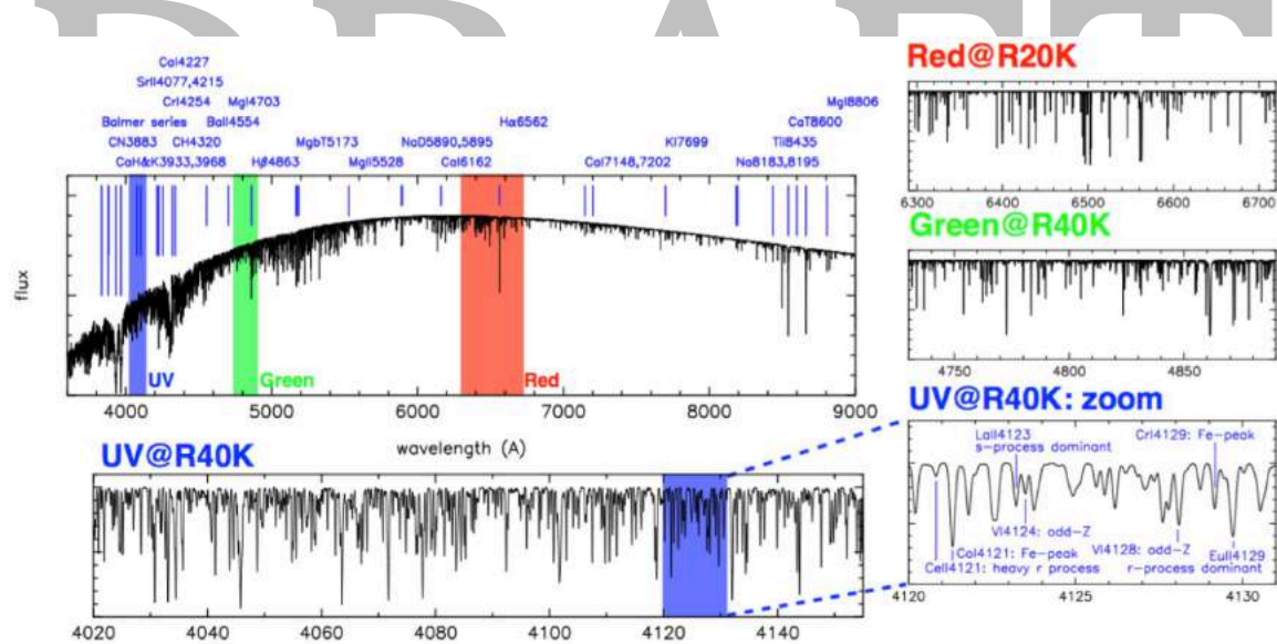
Figure 2: Main panel shows the relative flux of a synthetic spectrum of a metal poor red giant star at the intermediate MSE spectral resolution of R \sim 6000 , along with some of the strong line stellar diagnostics accessible at this resolution. Highlighted regions show the normalized flux in three windows observable with the high resolution mode of MSE. A magnified region of the UV window shows examples of the species that will be identified at high resolution. MSE chemical tagging surveys will identify species sampling a large and diverse set of nucleosynthetic pathways and processes. See Chapter 2 for more details.
